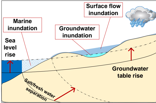
Fig. 1. Different sources of inundation
