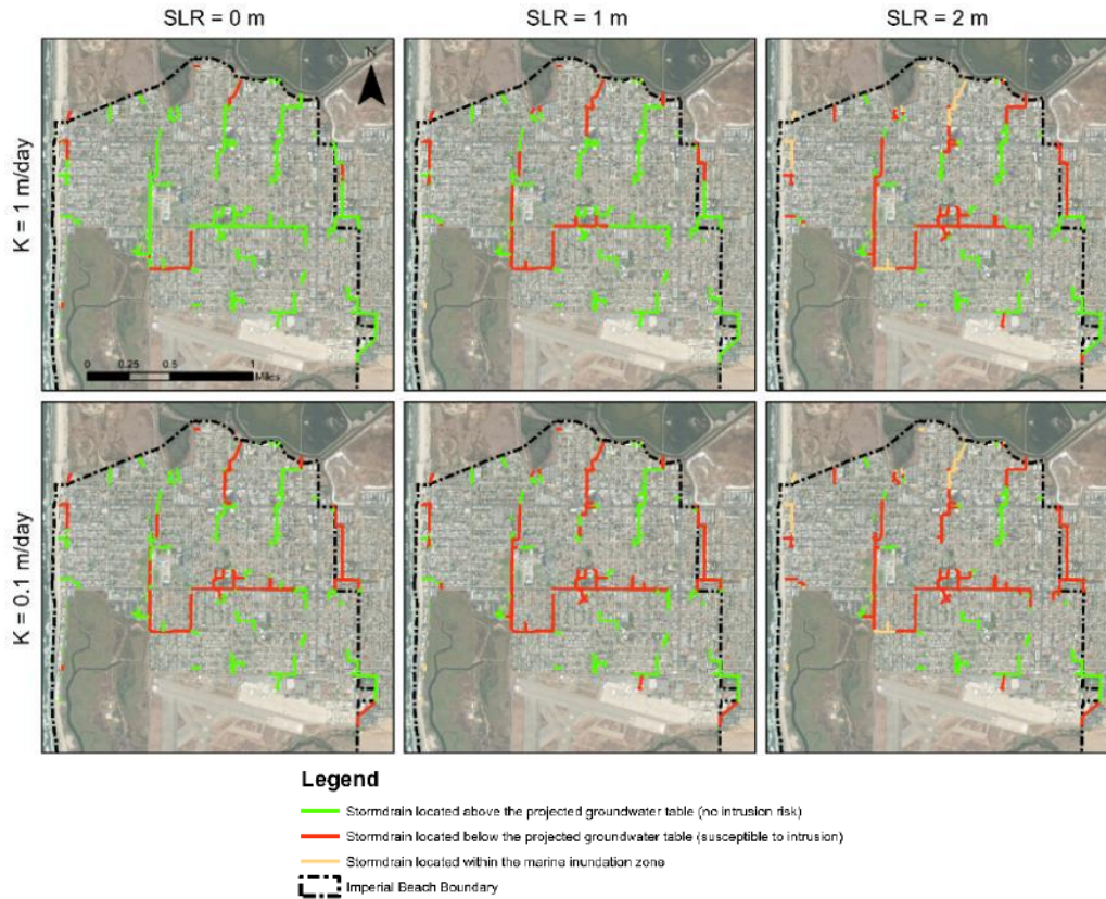
Fig. 4. Stormdrain analysis results
